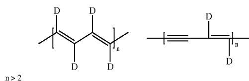
Scheme 1. Linear conjugated organic compounds and polymers
