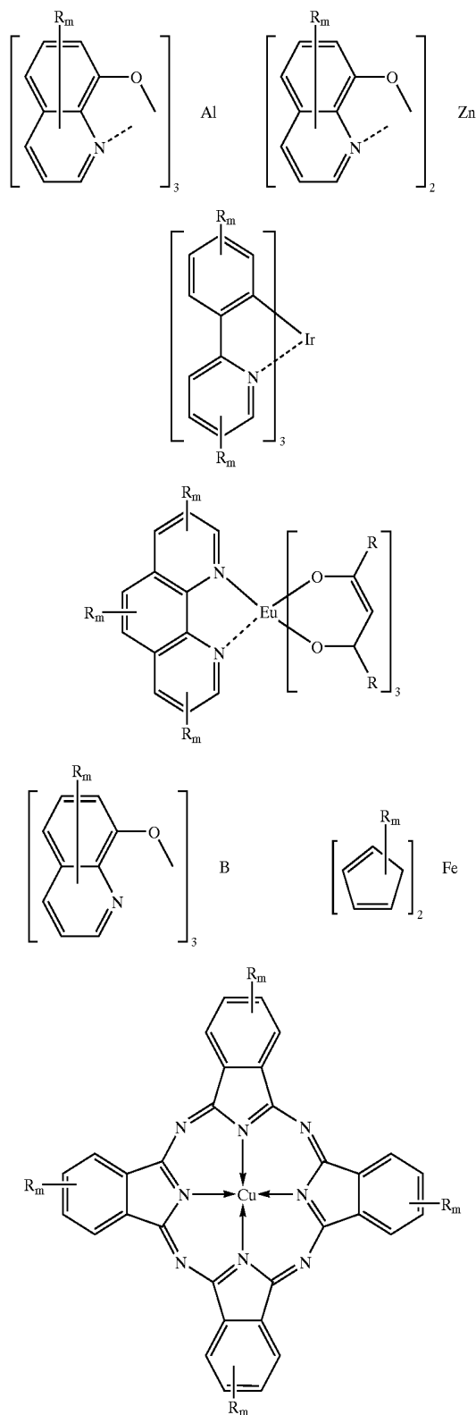
Scheme 4. Metal complexed organo-metallic compounds. (R: D, H, C 1 -C 30 alkyl, C 1 -C 30 alkoxy, C 1 -C 30 silyl, aryl, heteroaryl; m is 1-4).
