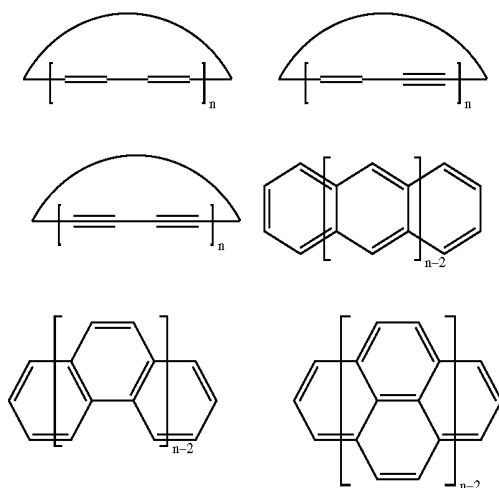
Scheme 2. Cyclic and fused ring combinations.
